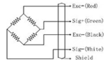
Wiring Schematic Diagram
